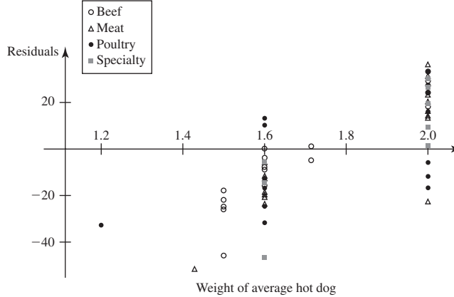
Figure 11.24 Plot of residuals against average hot dog weight. The points are labeled by the hot dog type.
